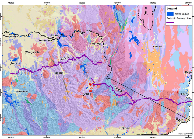
Fig 3. The geology of southeast Australia (source: Geoscience Australia). Colours correspond to different rock-types. Purple, blue and red rocks form the ancient 'bedrock'. Yellow rocks are younger sedimentary basins. Proposed survey routes are the dark purple lines.
