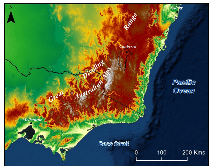
Fig 1. Elevation image of southeast Australia showing the Great Dividing Range and the Australian Alps.
